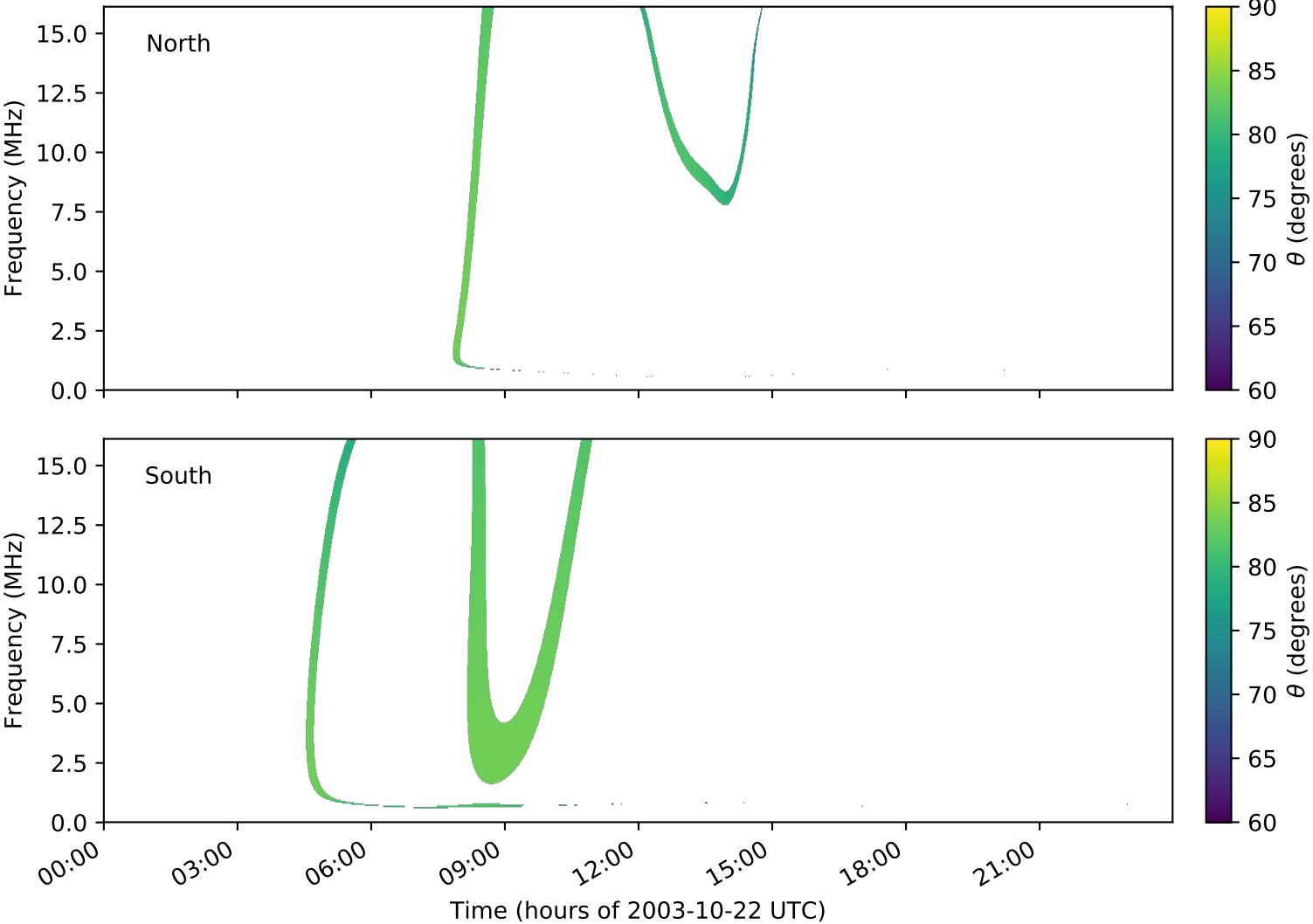
expres_cassini_jupiter_europa_isaac_lossc-wid1deg_3kev_20031022_v01.cdf
