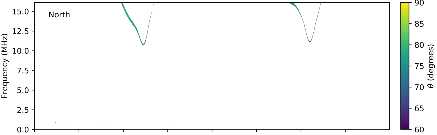
expres_cassini_jupiter_europa_isaac_lossc-wid1deg_3kev_20031019_v01.cdf
