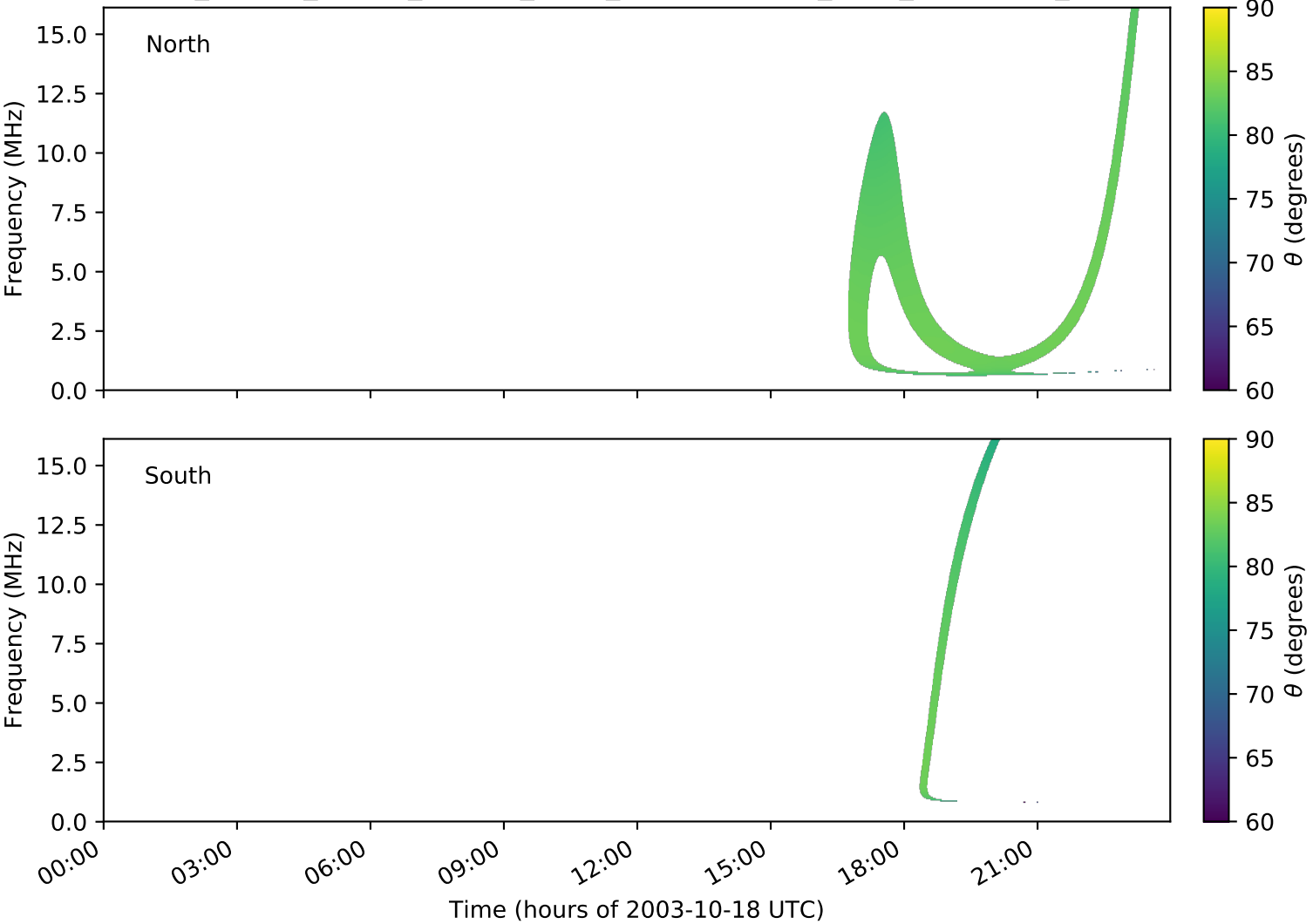
expres_cassini_jupiter_europa_isaac_lossc-wid1deg_3kev_20031018_v01.cdf
