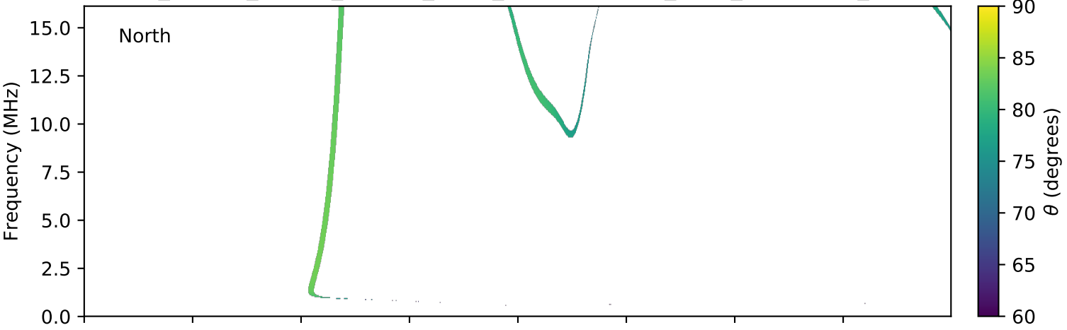
expres_cassini_jupiter_europa_isaac_lossc-wid1deg_3kev_20031015_v01.cdf
