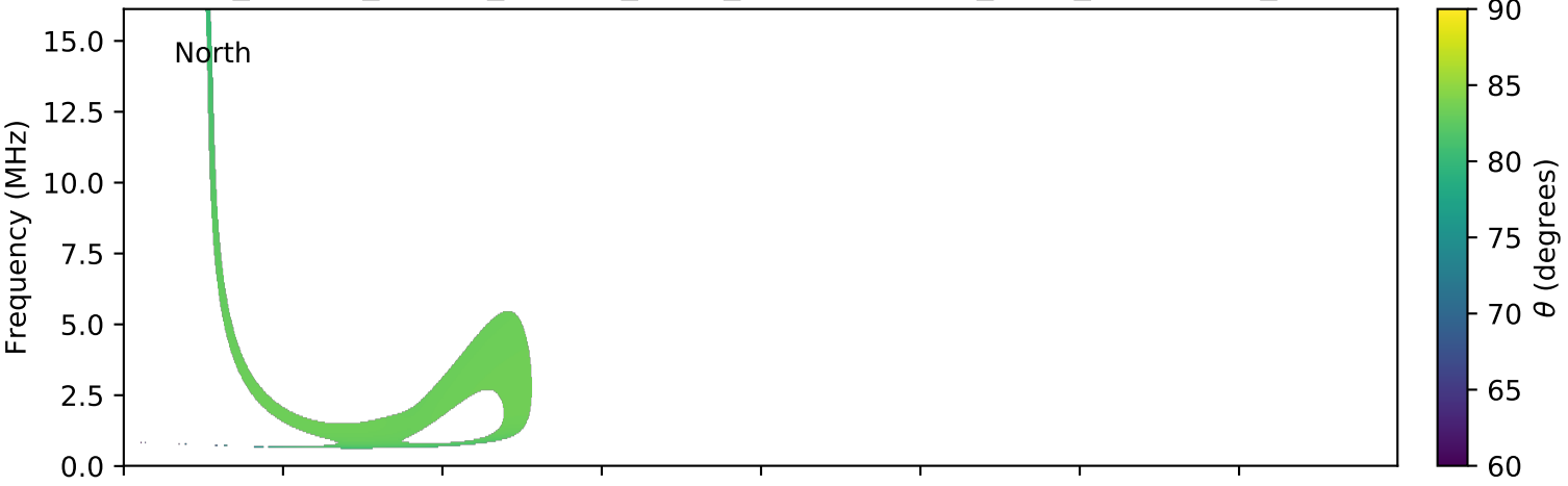
expres_cassini_jupiter_europa_isaac_lossc-wid1deg_3kev_20031013_v01.cdf
