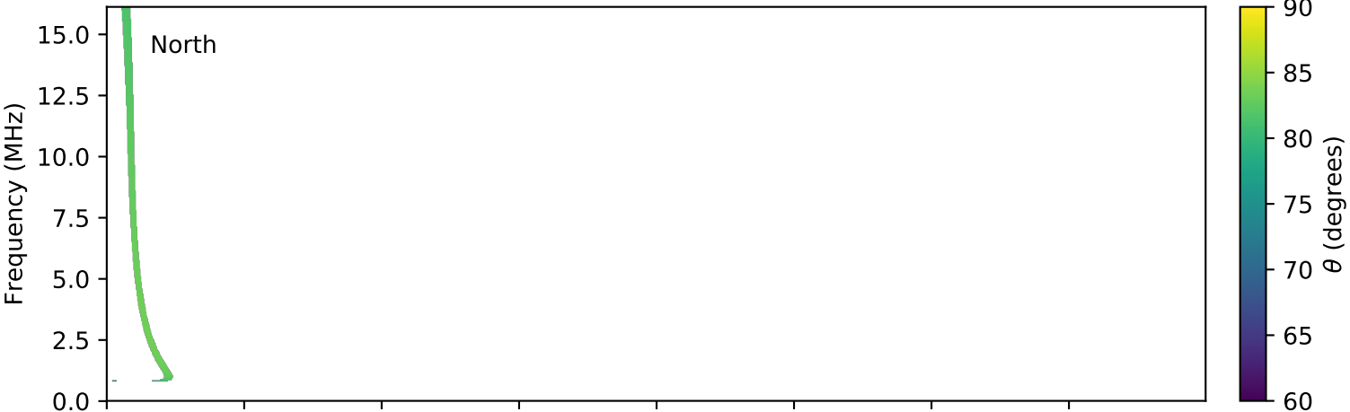
expres_cassini_jupiter_europa_isaac_lossc-wid1deg_3kev_20031006_v01.cdf
