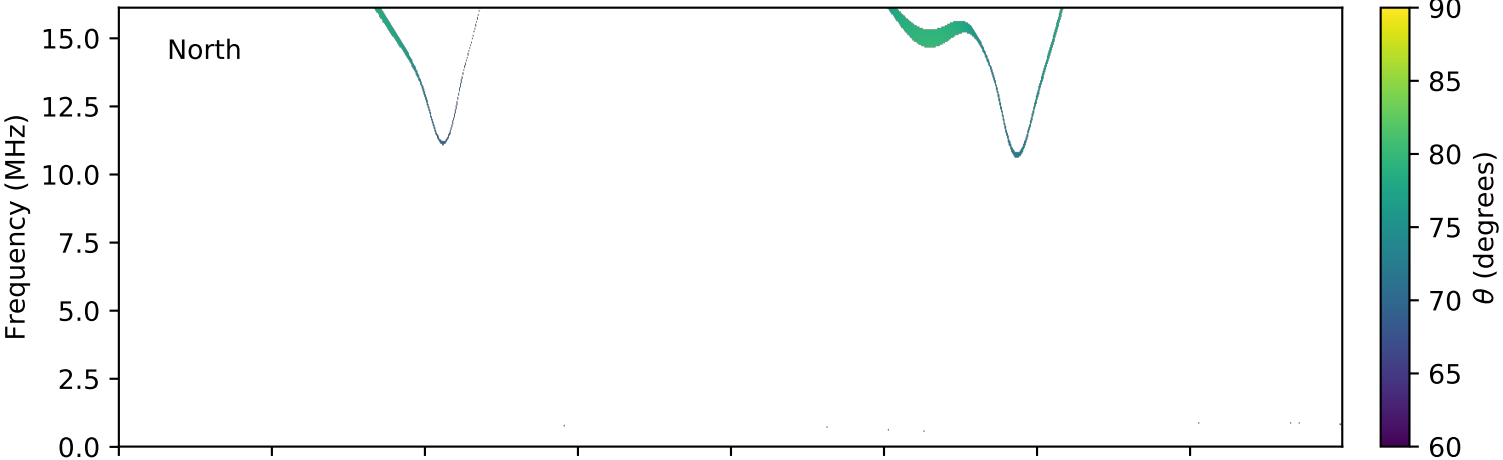
expres_cassini_jupiter_europa_isaac_lossc-wid1deg_3kev_20031005_v01.cdf
