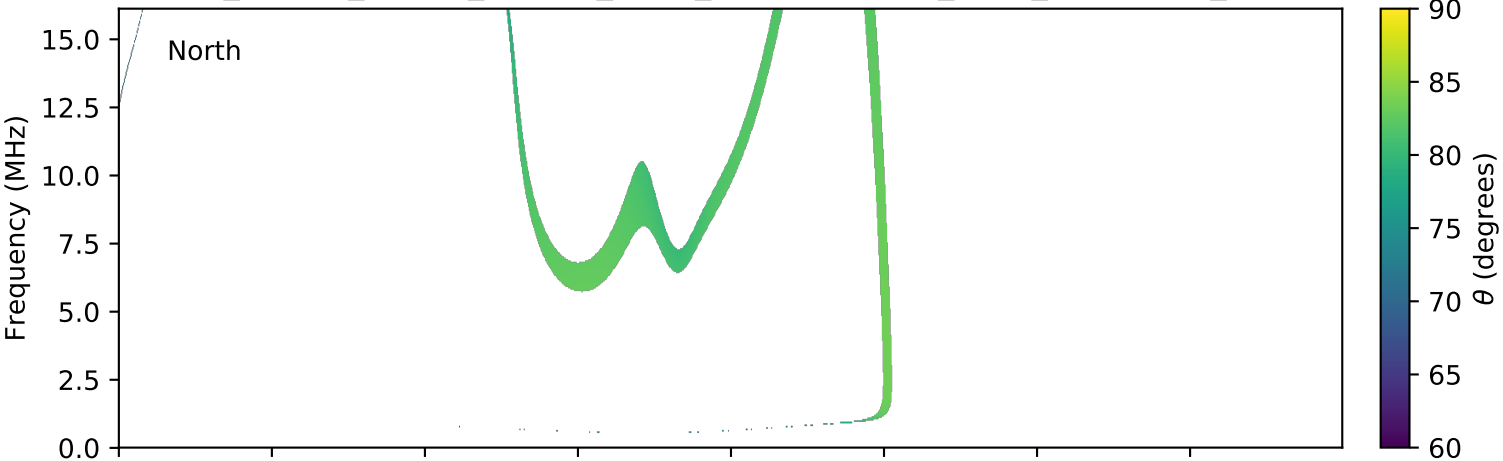
expres_cassini_jupiter_europa_isaac_lossc-wid1deg_3kev_20031002_v01.cdf
