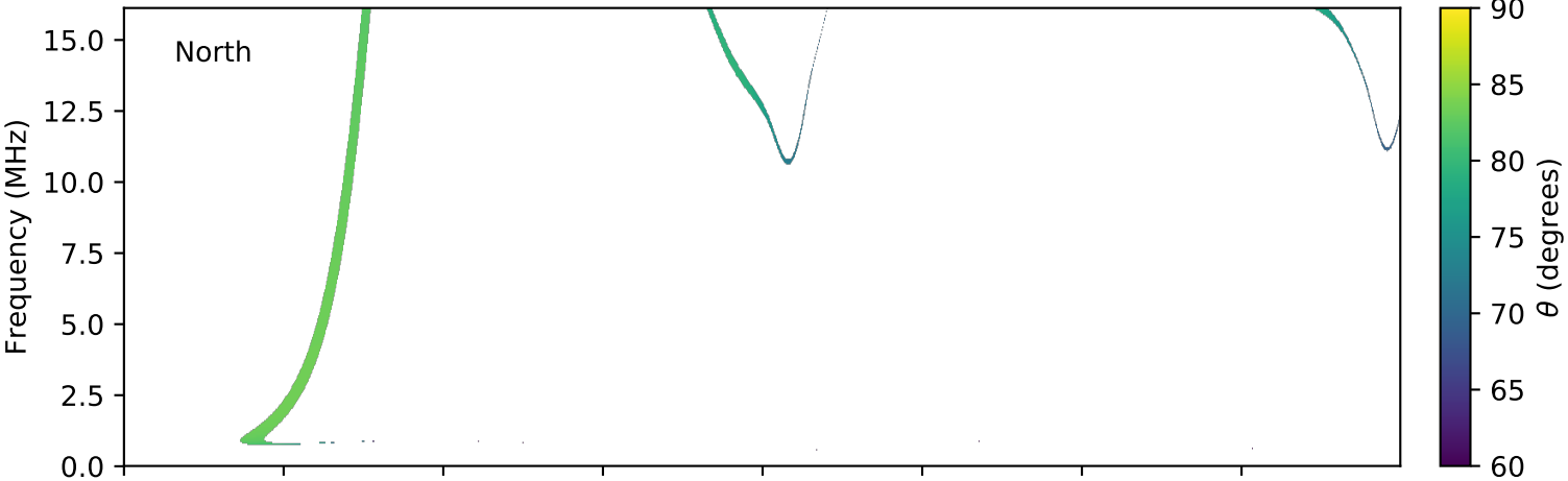
expres_cassini_jupiter_europa_isaac_lossc-wid1deg_3kev_20031001_v01.cdf
