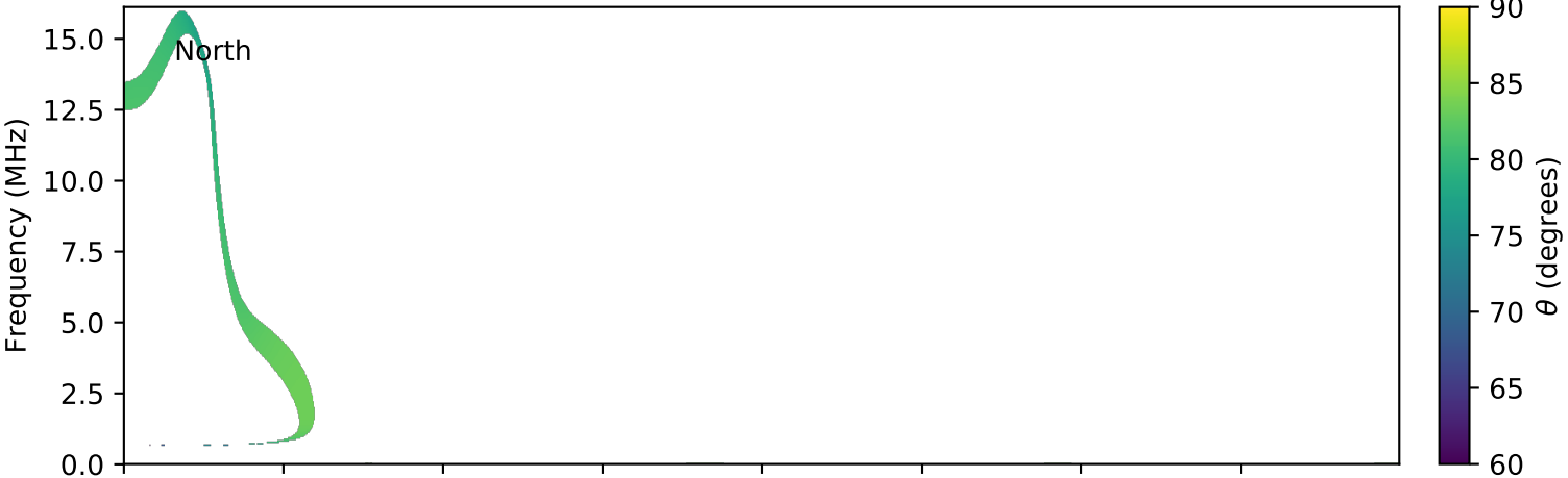
expres_cassini_jupiter_io_isaac_lossc-wid1deg_3kev_20030927_v01.cdf
