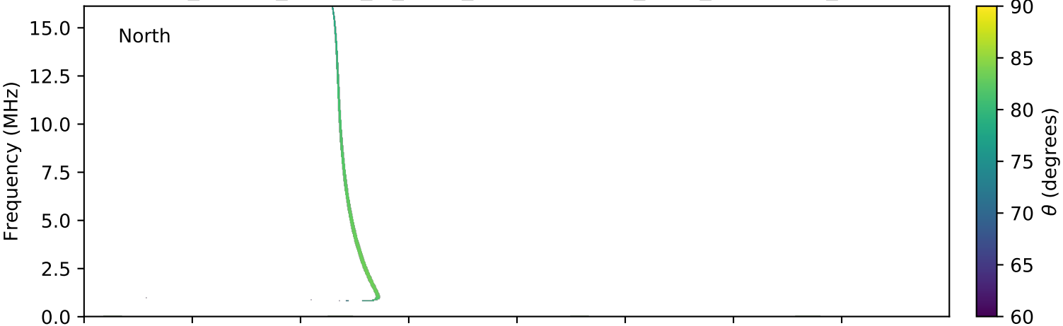
expres_cassini_jupiter_io_isaac_lossc-wid1deg_3kev_20030925_v01.cdf
