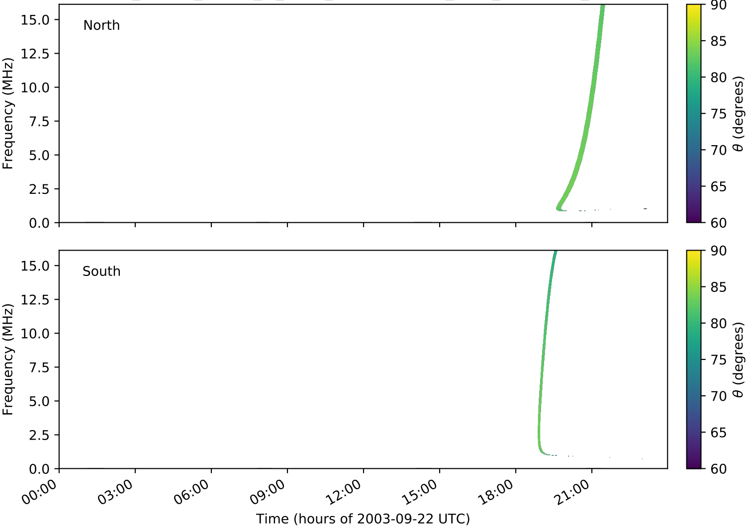
expres_cassini_jupiter_io_isaac_lossc-wid1deg_3kev_20030922_v01.cdf
