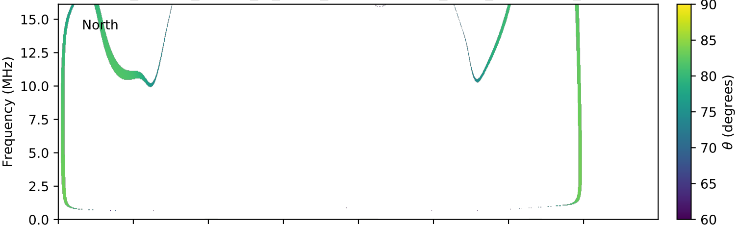
expres_cassini_jupiter_io_isaac_lossc-wid1deg_3kev_20030921_v01.cdf
