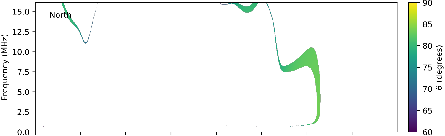
expres_cassini_jupiter_io_isaac_lossc-wid1deg_3kev_20030914_v01.cdf
