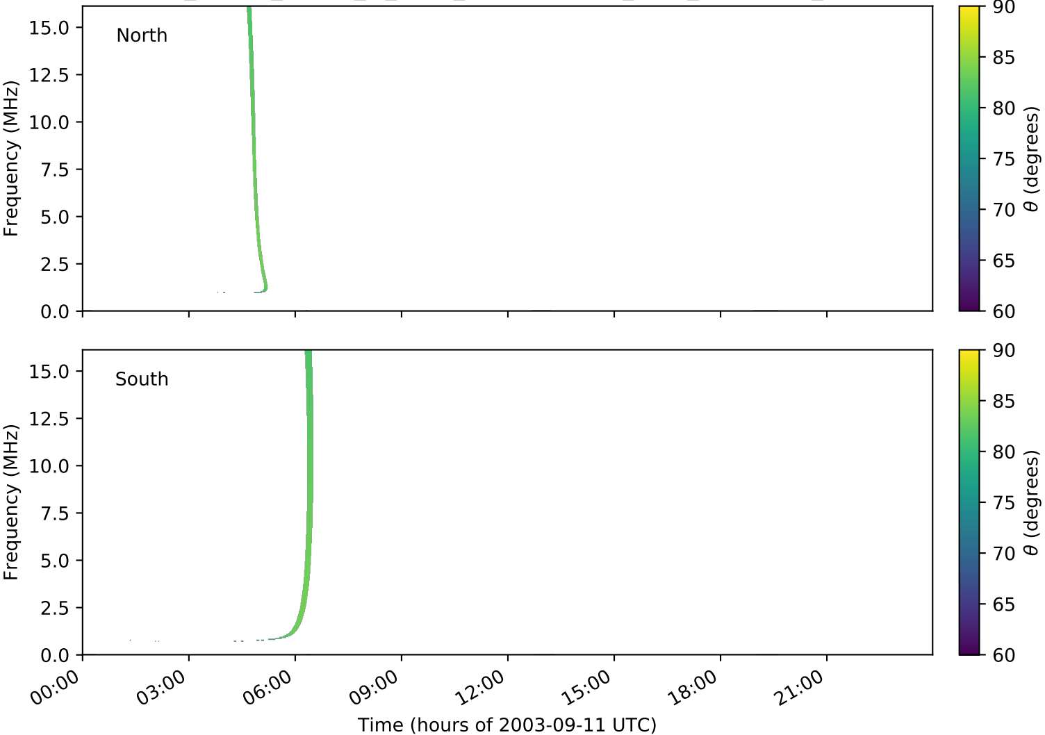
expres_cassini_jupiter_io_isaac_lossc-wid1deg_3kev_20030911_v01.cdf
