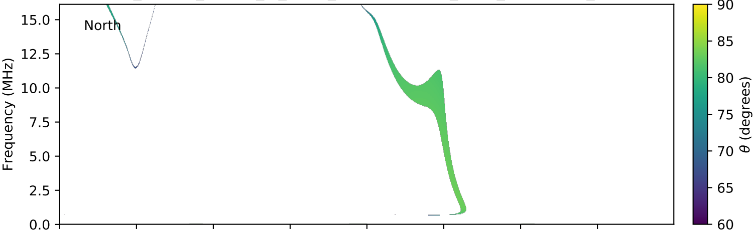
expres_cassini_jupiter_io_isaac_lossc-wid1deg_3kev_20030907_v01.cdf
