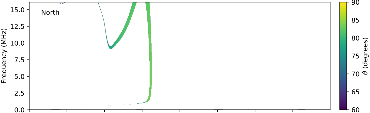
expres_cassini_jupiter_io_isaac_lossc-wid1deg_3kev_20030902_v01.cdf
