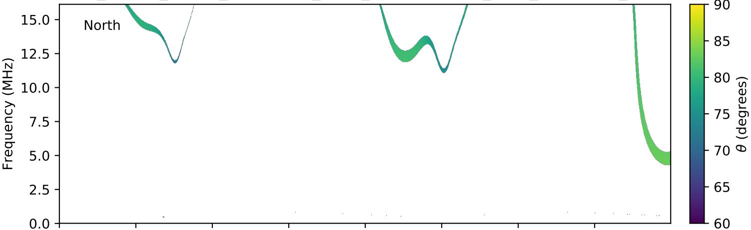
expres_cassini_jupiter_ganymede_isaac_lossc-wid1deg_3kev_20030926_v01.cdf
