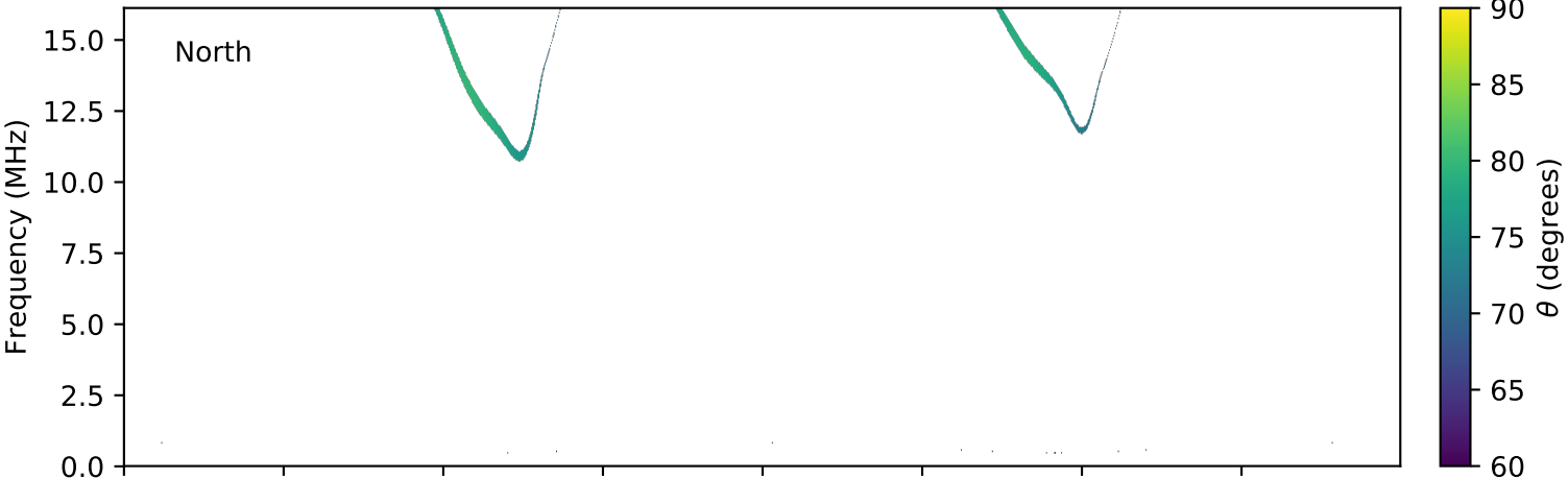
expres_cassini_jupiter_ganymede_isaac_lossc-wid1deg_3kev_20030925_v01.cdf
