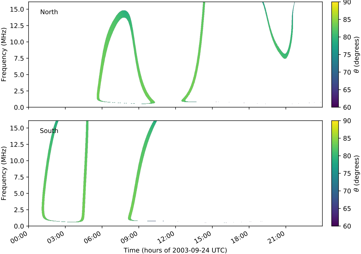
expres_cassini_jupiter_ganymede_isaac_lossc-wid1deg_3kev_20030924_v01.cdf
