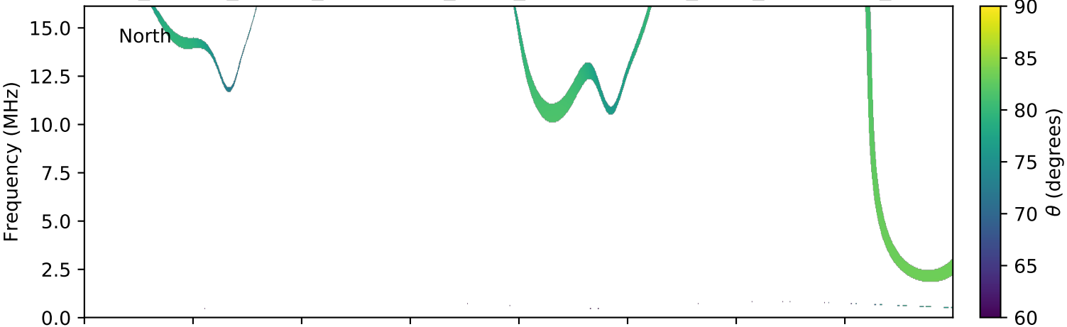
expres_cassini_jupiter_ganymede_isaac_lossc-wid1deg_3kev_20030919_v01.cdf
