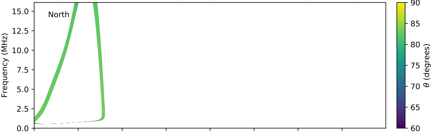
expres_cassini_jupiter_ganymede_isaac_lossc-wid1deg_3kev_20030913_v01.cdf
