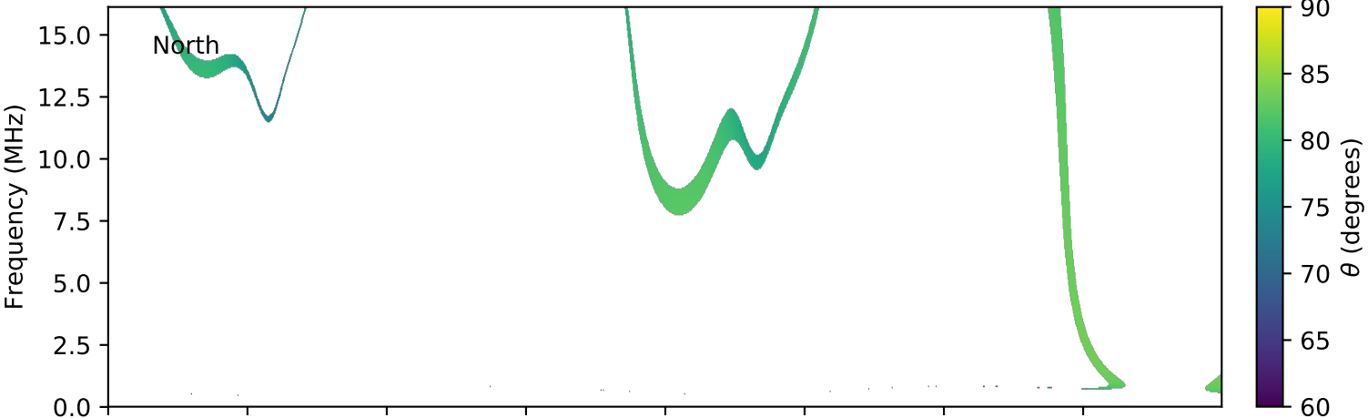
expres_cassini_jupiter_ganymede_isaac_lossc-wid1deg_3kev_20030912_v01.cdf
