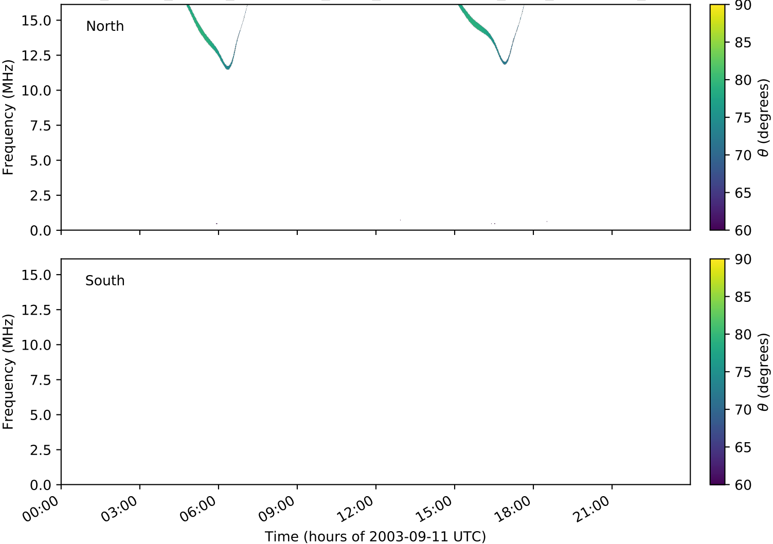
expres_cassini_jupiter_ganymede_isaac_lossc-wid1deg_3kev_20030911_v01.cdf
