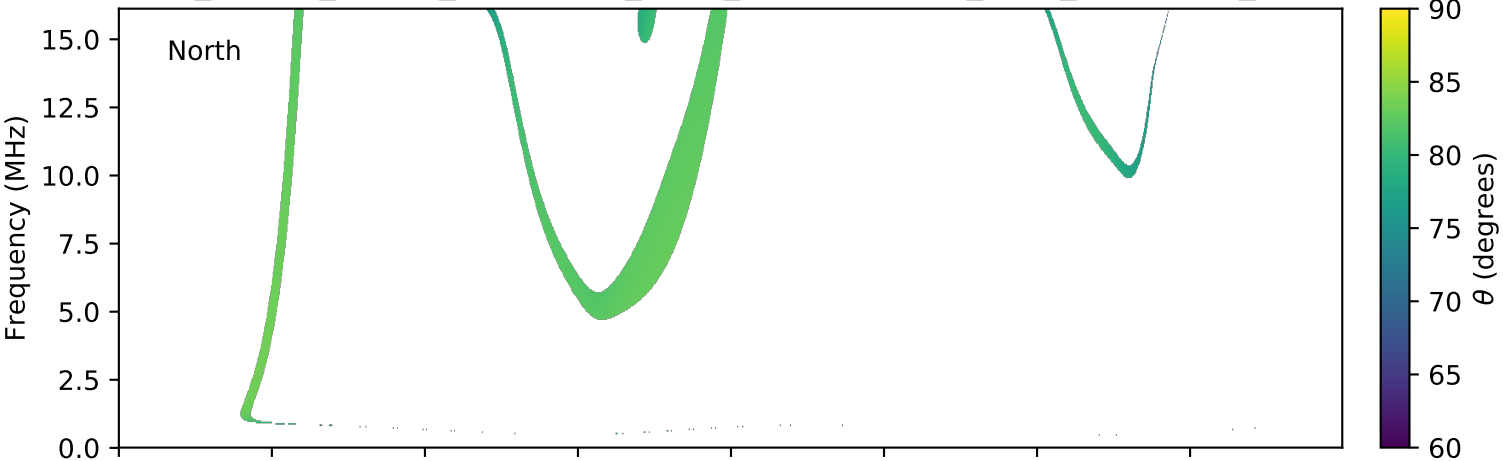
expres_cassini_jupiter_ganymede_isaac_lossc-wid1deg_3kev_20030910_v01.cdf
