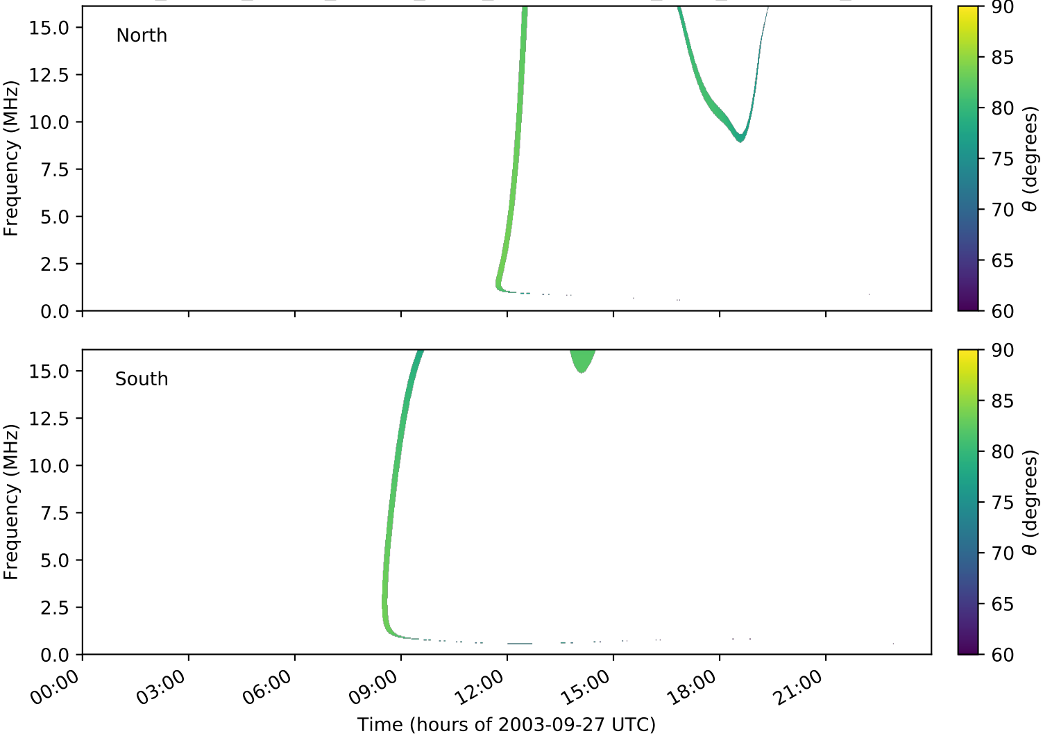
expres_cassini_jupiter_europa_isaac_lossc-wid1deg_3kev_20030927_v01.cdf
