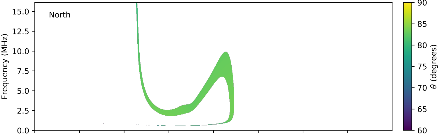
expres_cassini_jupiter_europa_isaac_lossc-wid1deg_3kev_20030925_v01.cdf
