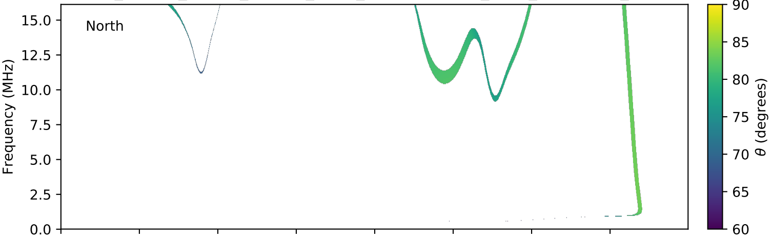
expres_cassini_jupiter_europa_isaac_lossc-wid1deg_3kev_20030921_v01.cdf
