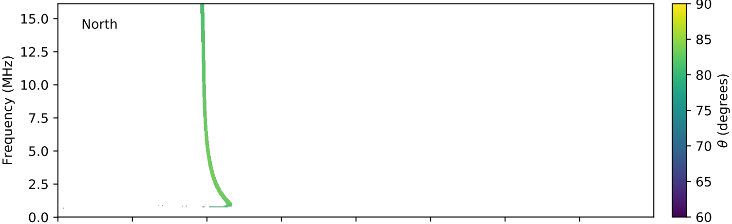
expres_cassini_jupiter_europa_isaac_lossc-wid1deg_3kev_20030918_v01.cdf
