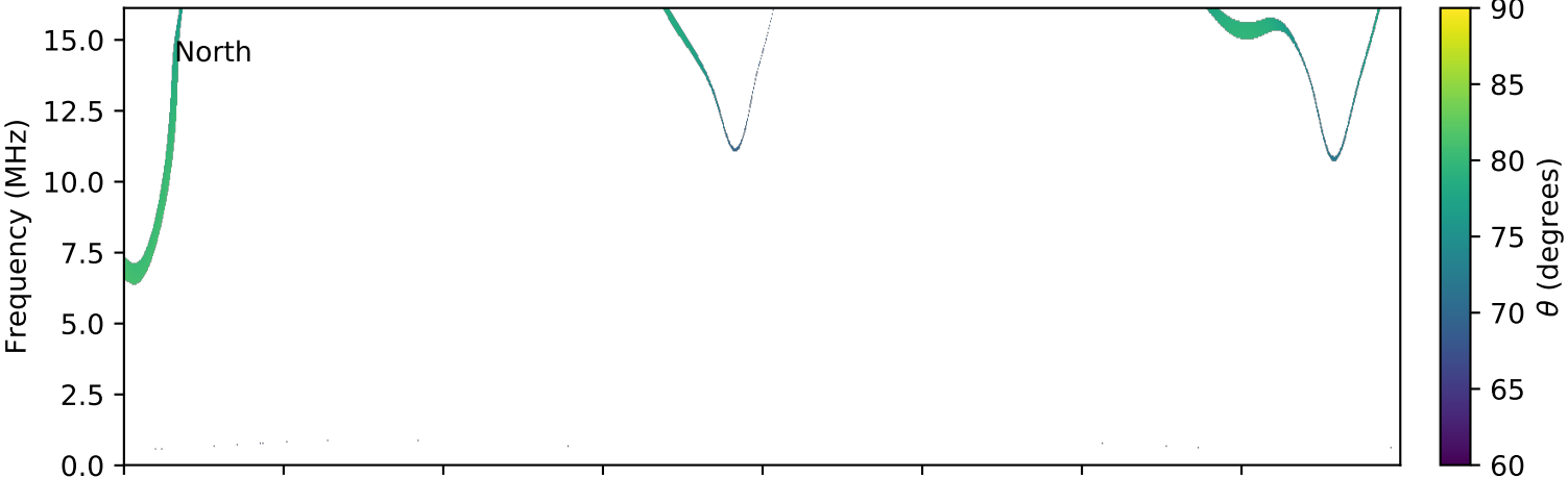
expres_cassini_jupiter_europa_isaac_lossc-wid1deg_3kev_20030917_v01.cdf
