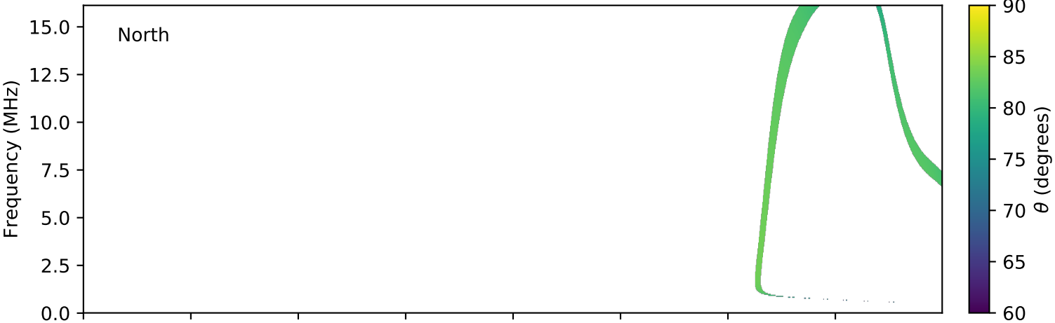
expres_cassini_jupiter_europa_isaac_lossc-wid1deg_3kev_20030916_v01.cdf
