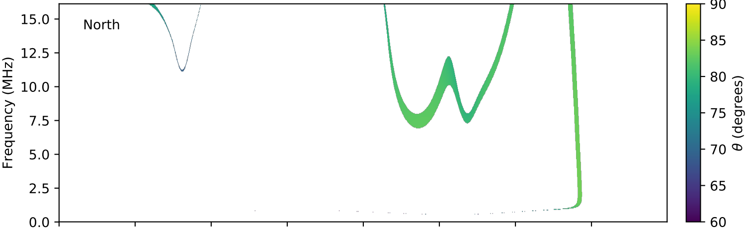
expres_cassini_jupiter_europa_isaac_lossc-wid1deg_3kev_20030914_v01.cdf
