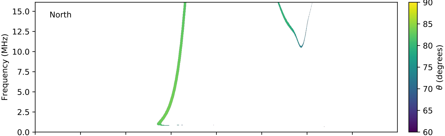
expres_cassini_jupiter_europa_isaac_lossc-wid1deg_3kev_20030913_v01.cdf
