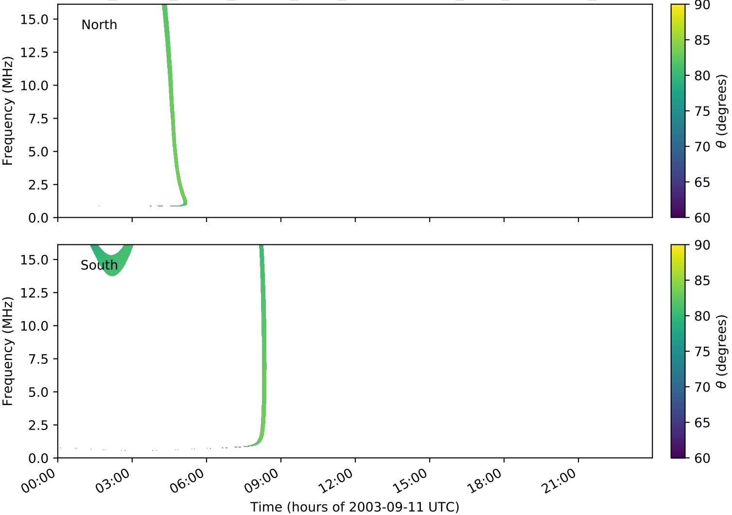
expres_cassini_jupiter_europa_isaac_lossc-wid1deg_3kev_20030911_v01.cdf
