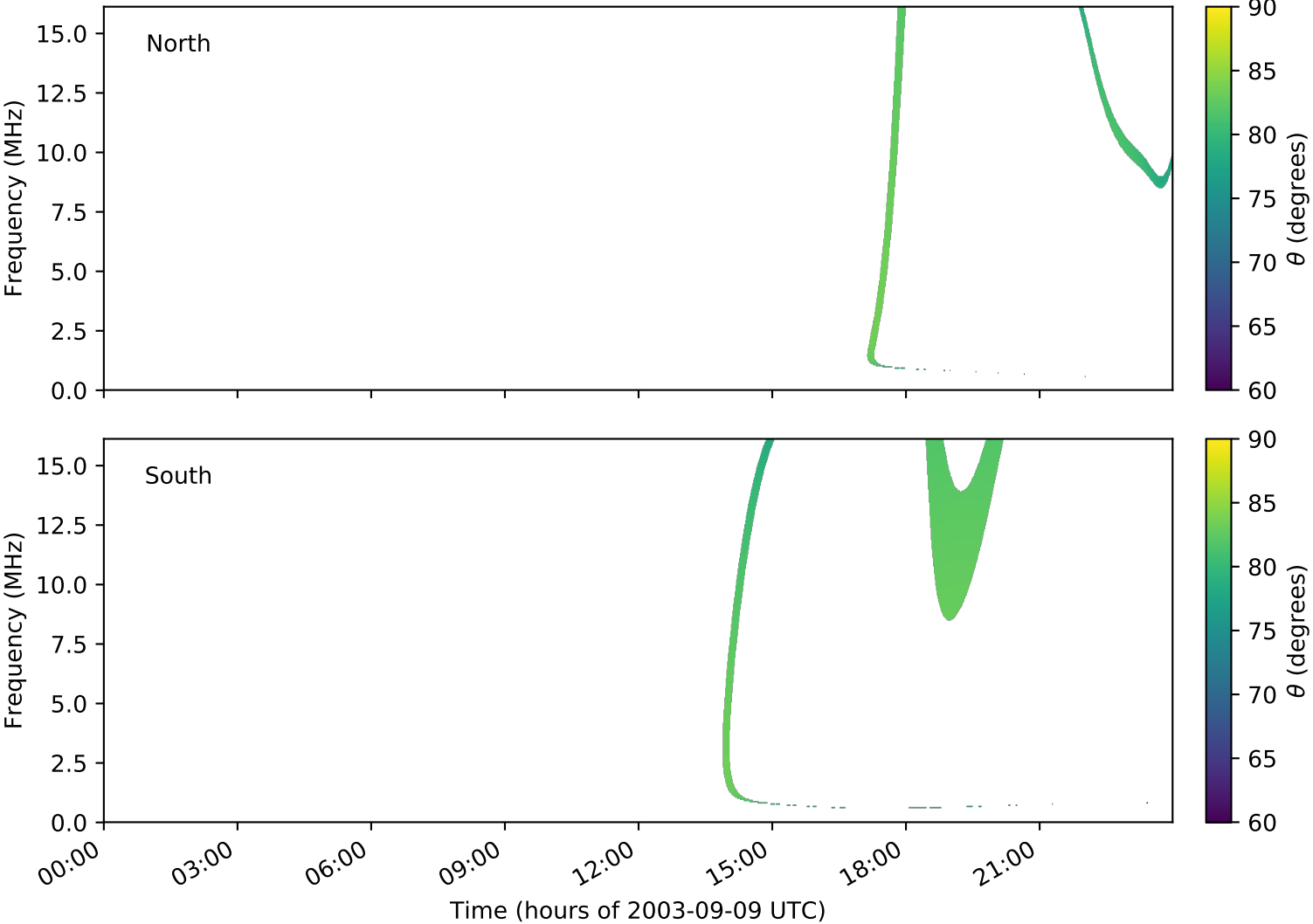
expres_cassini_jupiter_europa_isaac_lossc-wid1deg_3kev_20030909_v01.cdf
