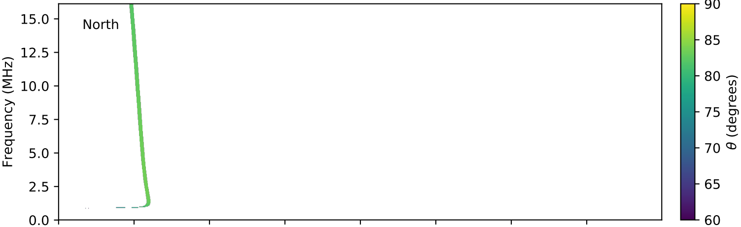
expres_cassini_jupiter_europa_isaac_lossc-wid1deg_3kev_20030904_v01.cdf
