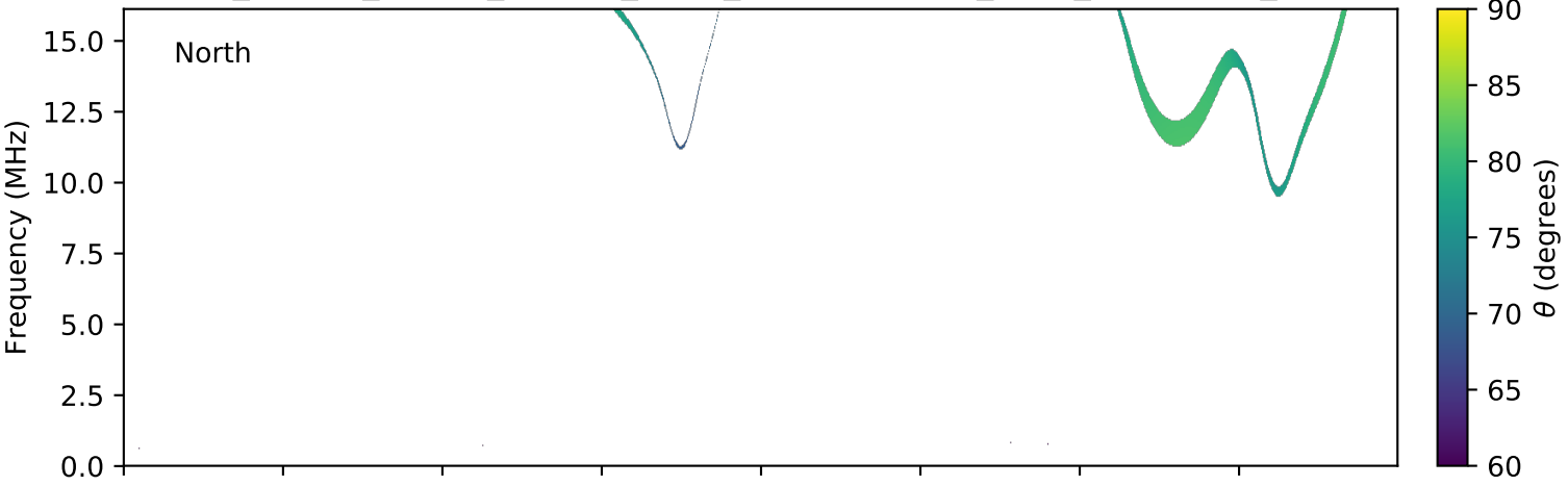
expres_cassini_jupiter_europa_isaac_lossc-wid1deg_3kev_20030903_v01.cdf
