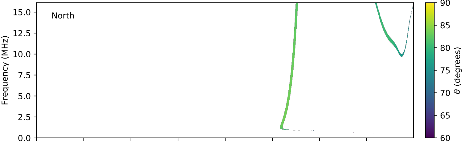
expres_cassini_jupiter_europa_isaac_lossc-wid1deg_3kev_20030902_v01.cdf
