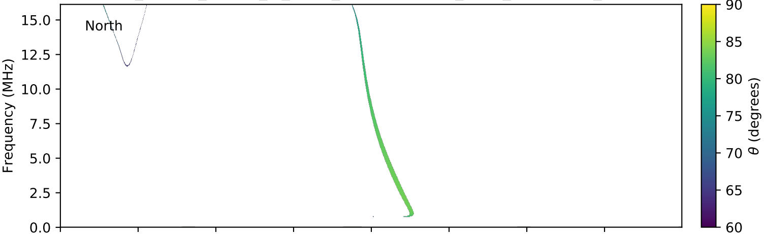
expres_cassini_jupiter_io_isaac_lossc-wid1deg_3kev_20030831_v01.cdf
