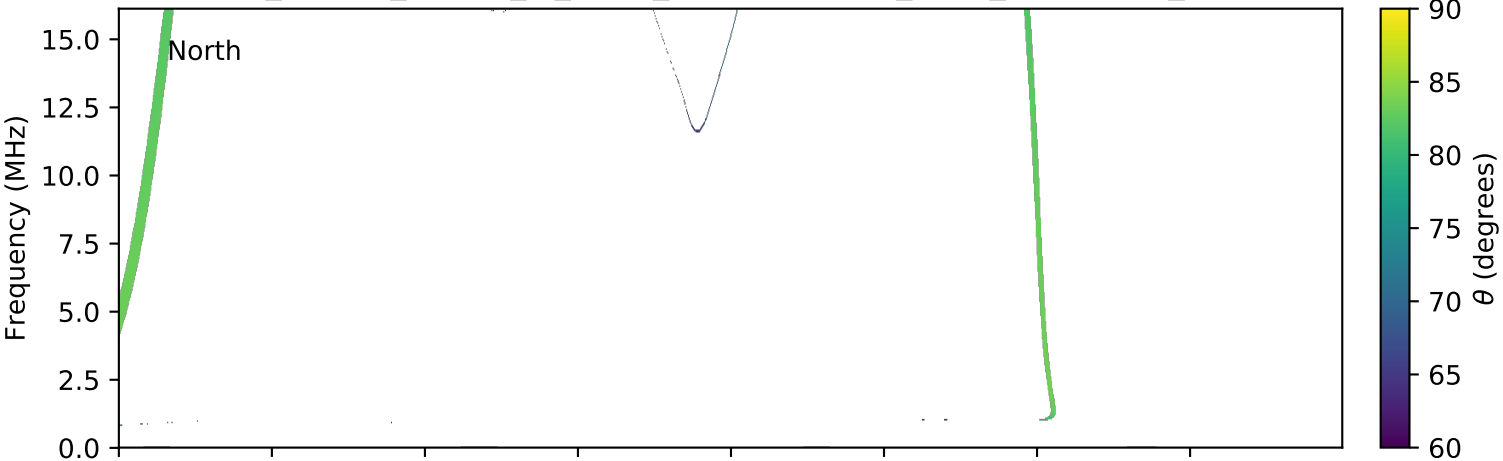
expres_cassini_jupiter_io_isaac_lossc-wid1deg_3kev_20030822_v01.cdf
