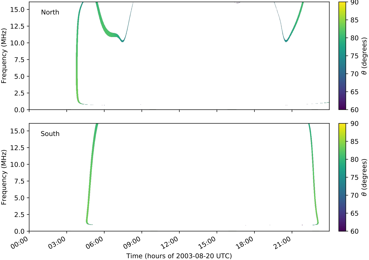
expres_cassini_jupiter_io_isaac_lossc-wid1deg_3kev_20030820_v01.cdf
