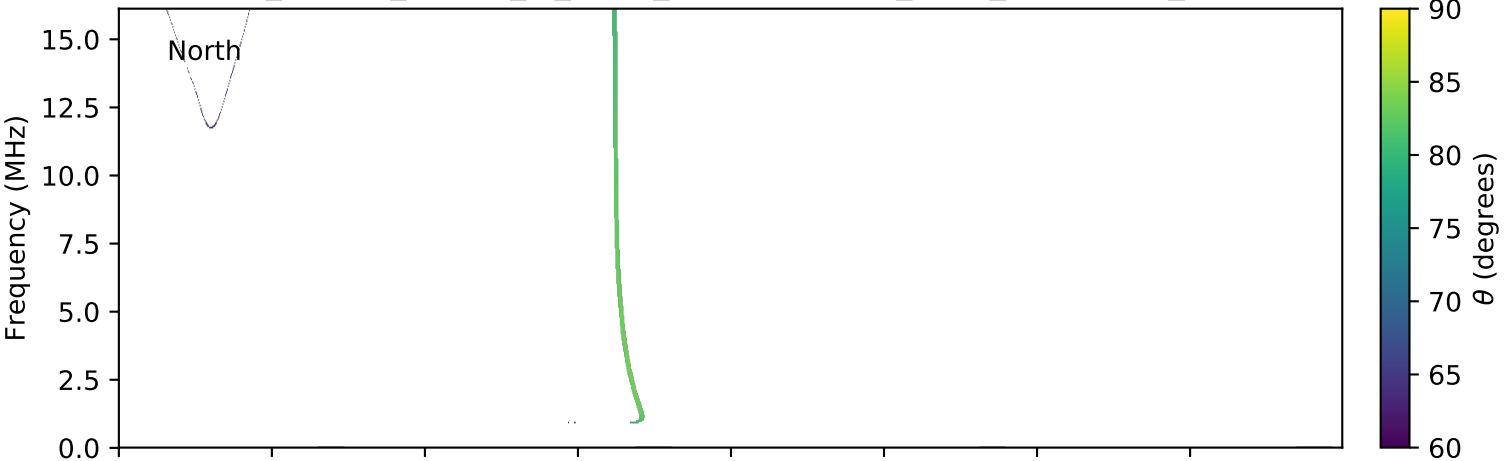
expres_cassini_jupiter_io_isaac_lossc-wid1deg_3kev_20030817_v01.cdf
