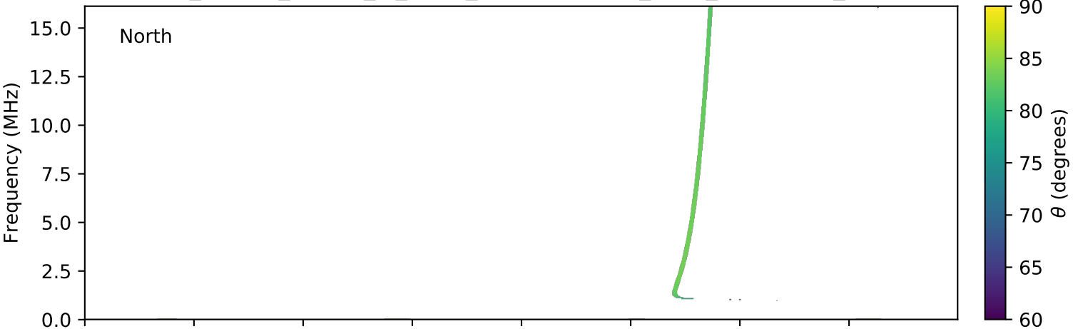
expres_cassini_jupiter_io_isaac_lossc-wid1deg_3kev_20030816_v01.cdf
