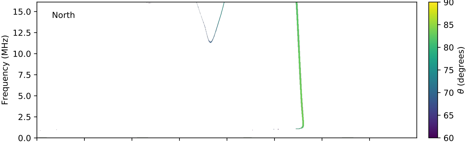
expres_cassini_jupiter_io_isaac_lossc-wid1deg_3kev_20030815_v01.cdf
