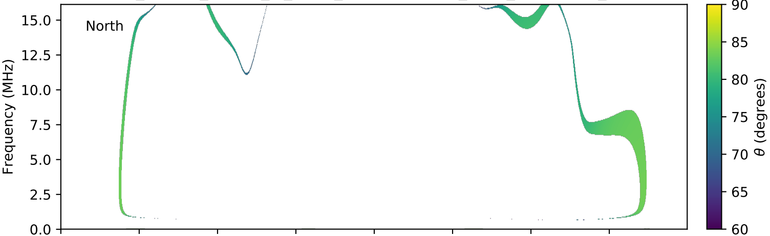
expres_cassini_jupiter_io_isaac_lossc-wid1deg_3kev_20030813_v01.cdf
