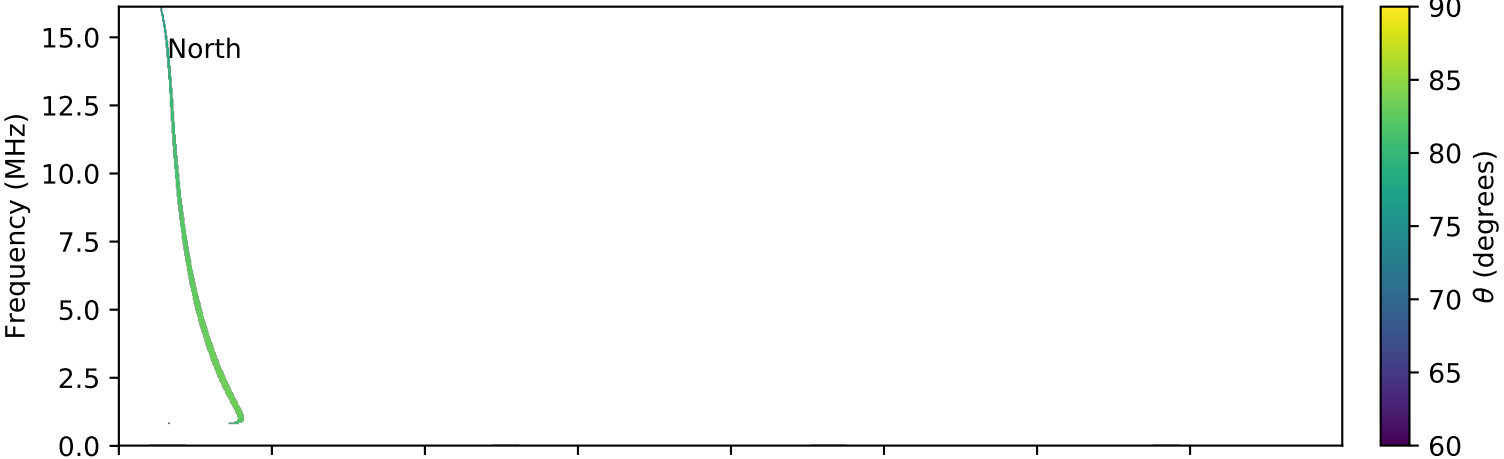
expres_cassini_jupiter_io_isaac_lossc-wid1deg_3kev_20030812_v01.cdf
