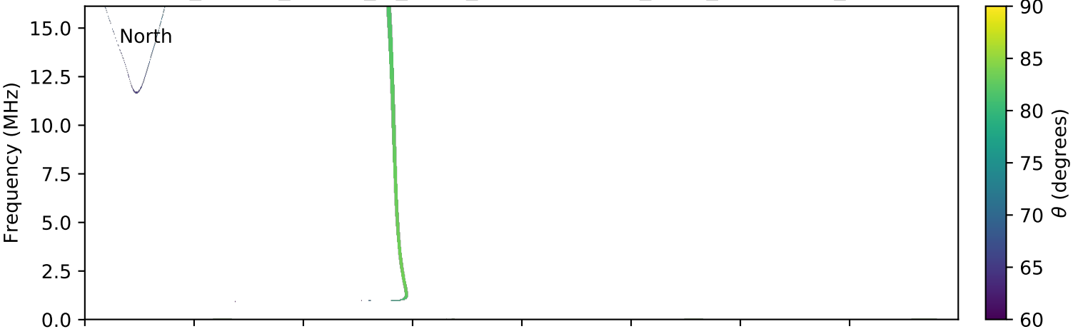
expres_cassini_jupiter_io_isaac_lossc-wid1deg_3kev_20030810_v01.cdf
