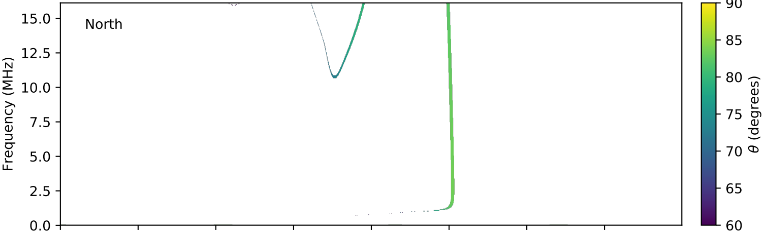
expres_cassini_jupiter_io_isaac_lossc-wid1deg_3kev_20030808_v01.cdf
