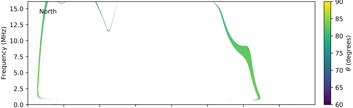
expres_cassini_jupiter_io_isaac_lossc-wid1deg_3kev_20030806_v01.cdf
