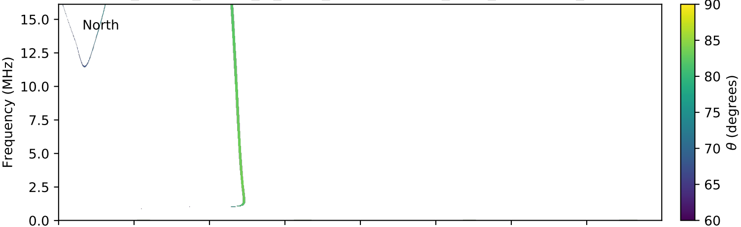
expres_cassini_jupiter_io_isaac_lossc-wid1deg_3kev_20030803_v01.cdf
